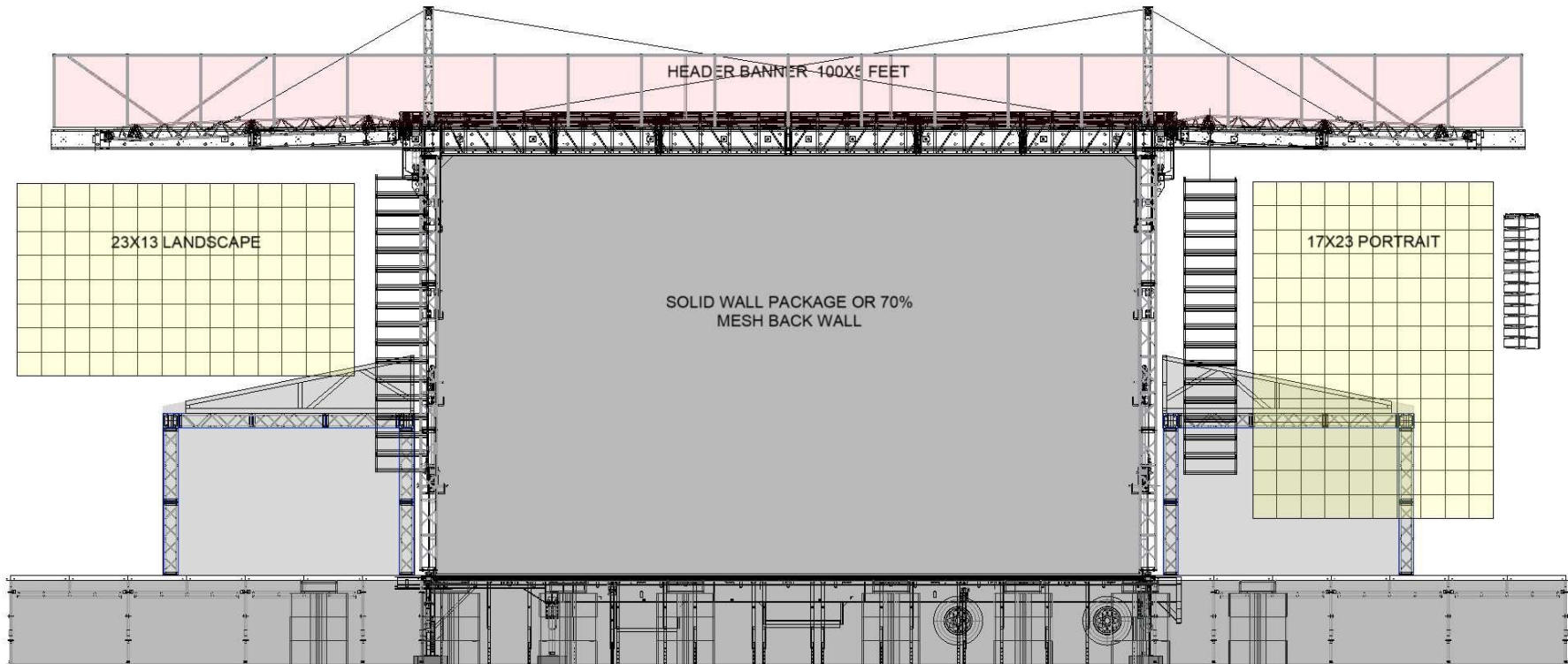
EXAMPLE #1 PA ON FRONT HANG POINTS, LANDSCAPE
